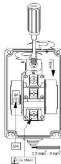
Adjusting the flow switch's triac sensitivity
